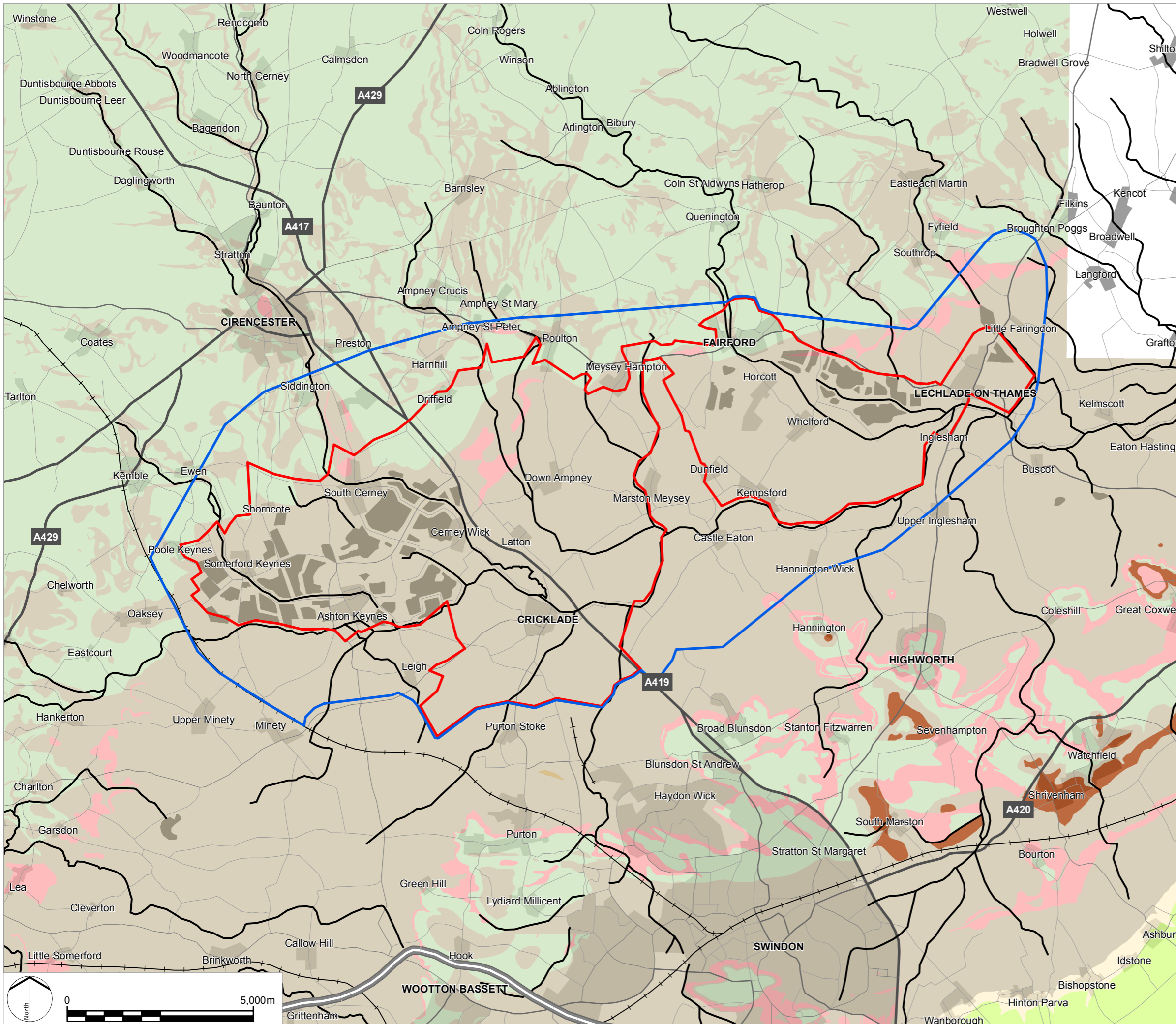
Figure 6: Bedrock Geology
