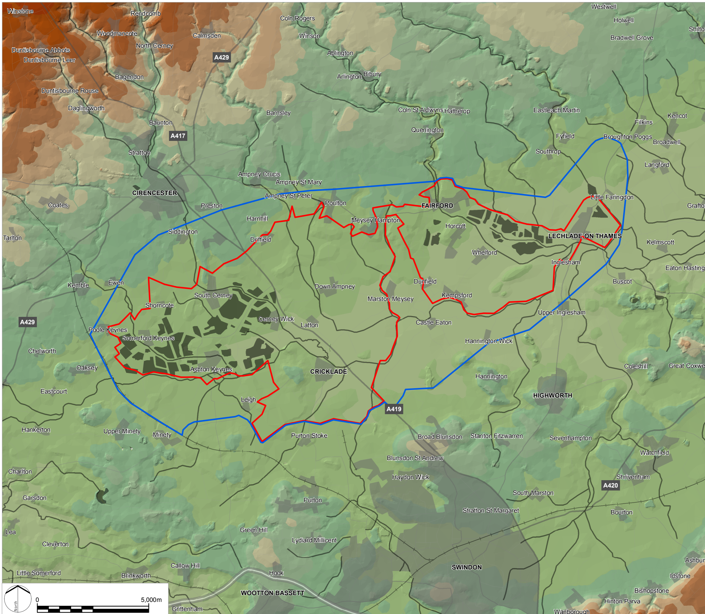
Figure 7: Landform
